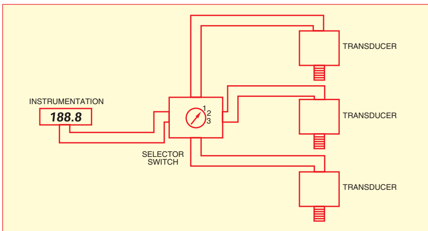
Figure 6: Multiple transducers wired to one meter and one switch (transducers with built-in zero & span adjustments, same outputs & same pressure ranges)
