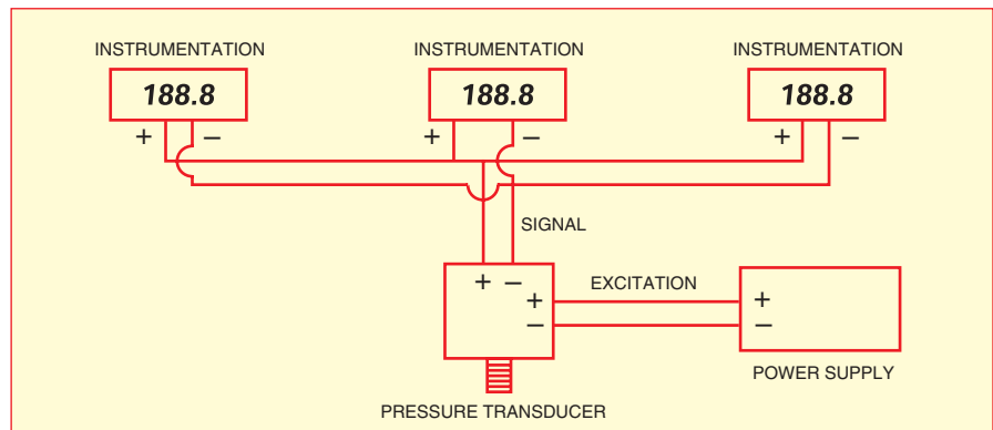
Figure 5: Multiple instruments wired in parallel to a voltage output transducer
