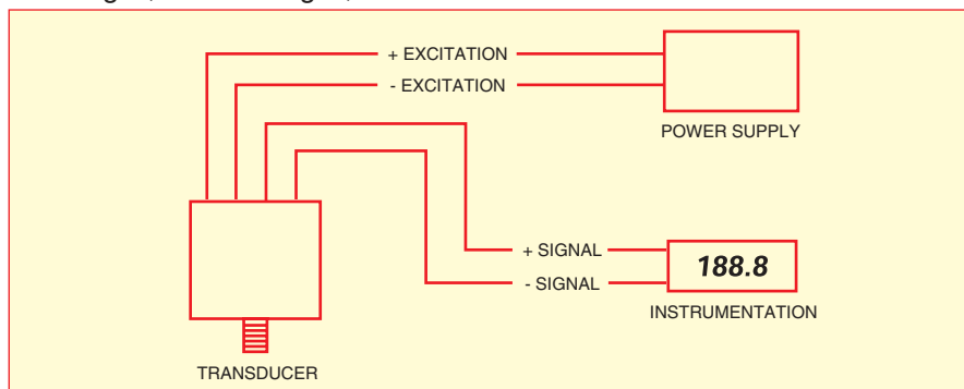
Figure 1: Typical wiring configuration for millivolt output transducer
