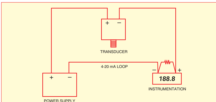
Figure 7: Converting current into voltage for instrumentation set up for voltage
