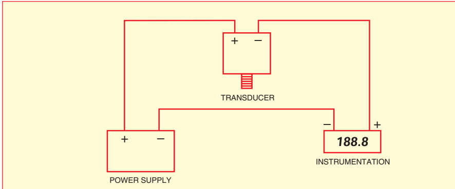
Figure 3: Typical wiring configuration for current output transducer
