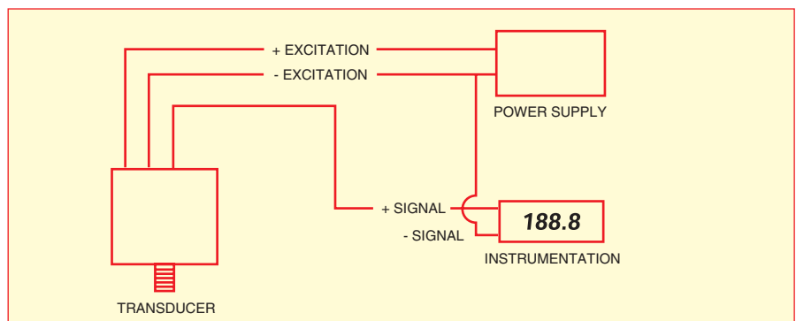
Figure 2: Typical wiring configuration for voltage output transducer (-excitation and -signal are common)
