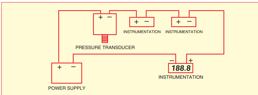
Figure 4: Multi-instrument 4-20 mA current loop (panel meters, chart recorder, computers, etc.)
